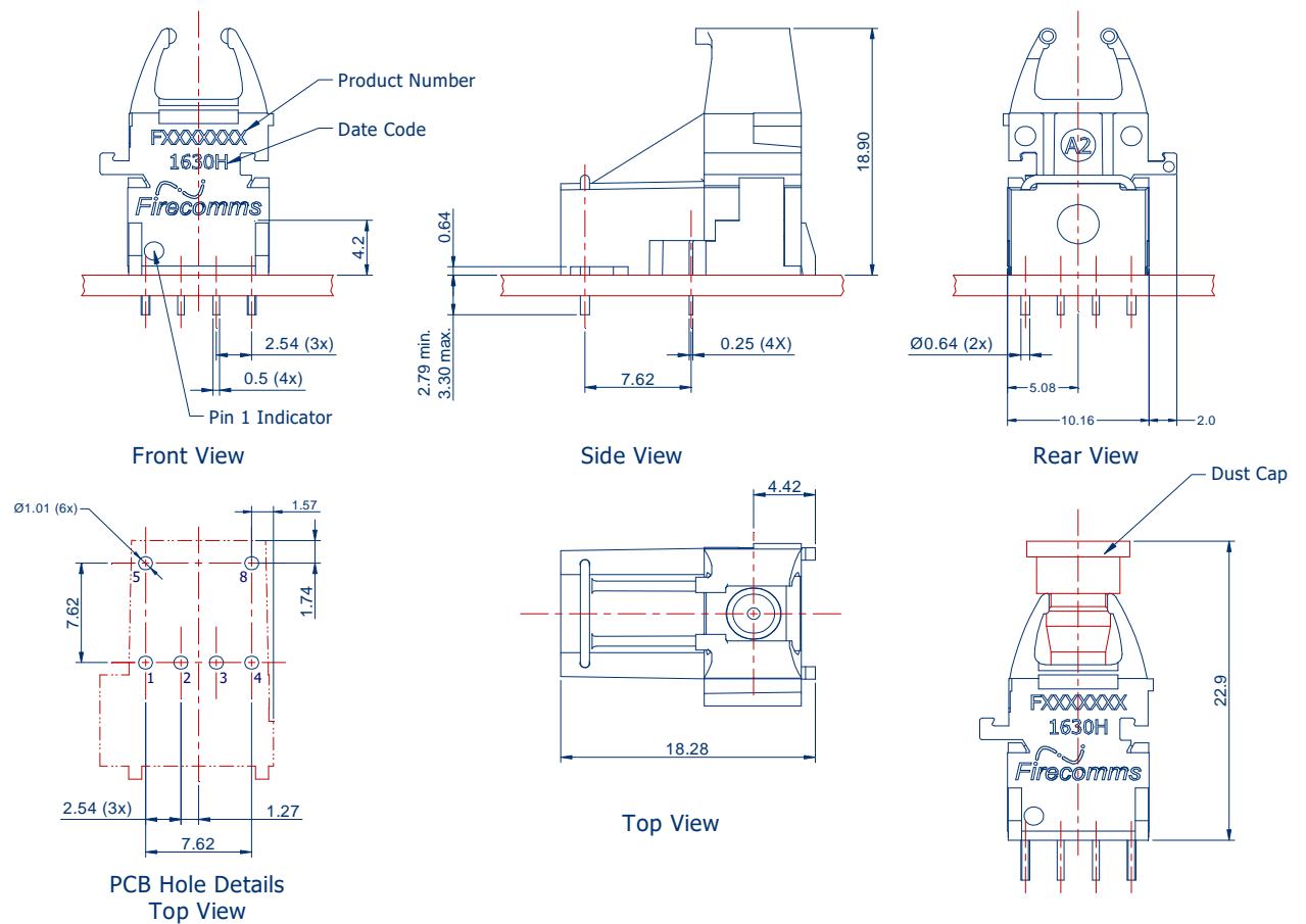
FIGURE 11 Mechanical dimensions of the vertical transmitter connectors and PCB footprint, which is a top view General dimensional tolerance is \pm 0.2 mm
