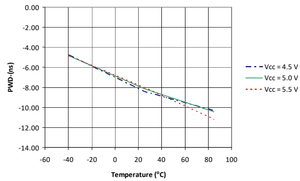
FIGURE 7 Typical pulse width distortion vs. temperature.
